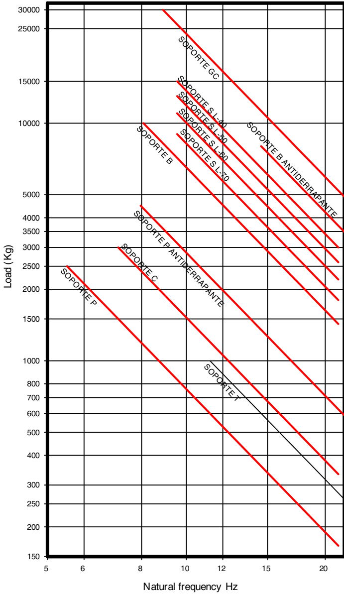
NATURAL FREQUENCIES A MC MECANOCAUCHO® Type G.C.
