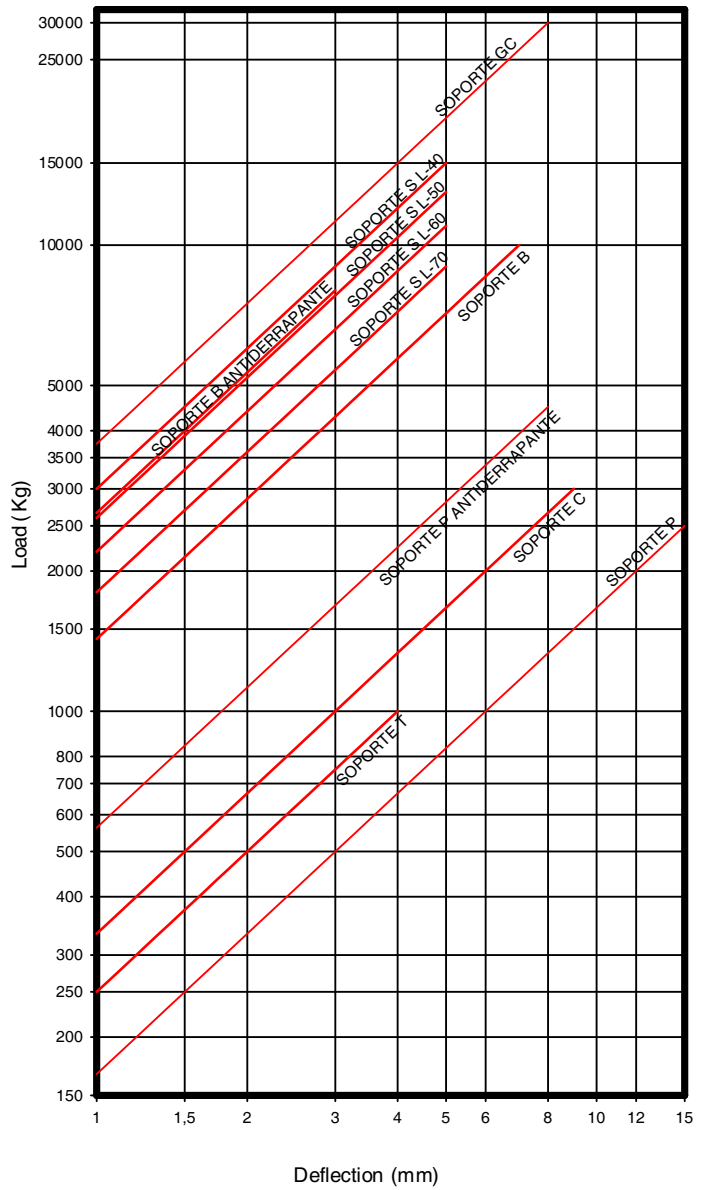
LOAD DEFLECTION GRAPHS MECANOCAUCHO® Type G.C.
