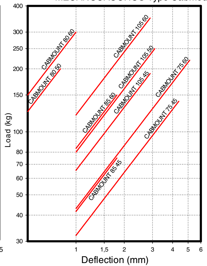
LOAD DEFLECTION GRAPHS MECANOCAUCHO® Type Cabmount
