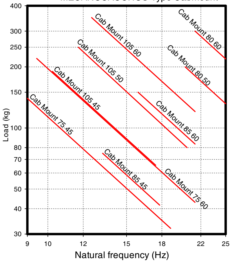
NATURAL FREQUENCIES AMC MECANOCAUCHO® Type Cabmount
