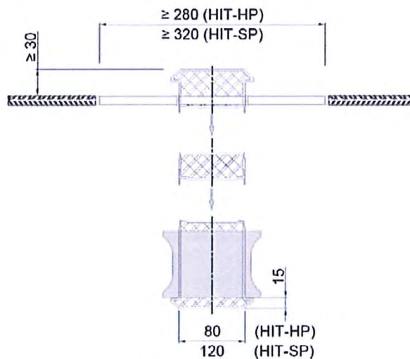
Figure 13: Halfen Insulated Connection HIT-HP/SP multi-part execution variation
