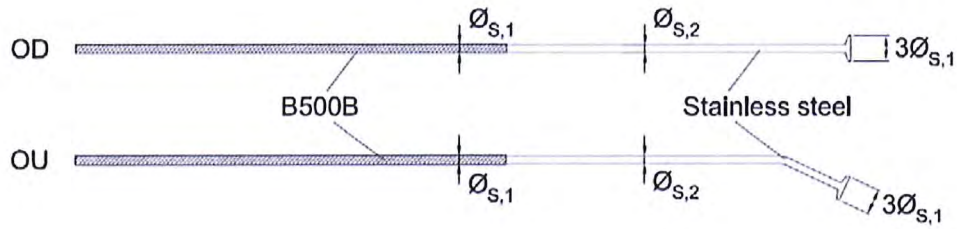
Figure 15: Tension bar variations Halfen Insulated Connection HIT-HP/SP MVX OU/OD (embedment length of stainless steel of \geq 10\text{cm} in the adjacent concrete)
