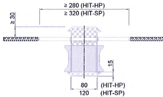
Figure 11: Halfen Insulated Connection HIT-HP/SP completed execution variation
