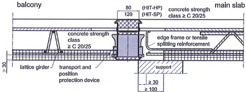
Figure 19: Example of the connection HIT-HP/SP MVX to element slabs with statically effective in-situ layer
