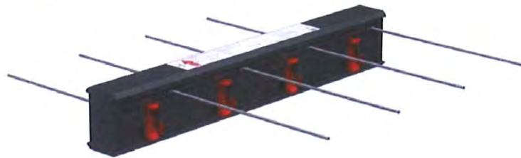
Figure 5: Halfen Insulated Connection HIT-HP/SP ZVX
