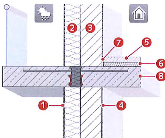
Figure 31: Wall construction with ETICS
