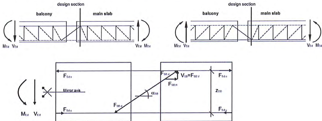
Figure 39: Strut-and-tie model and design section HIT-HP/SP DD
