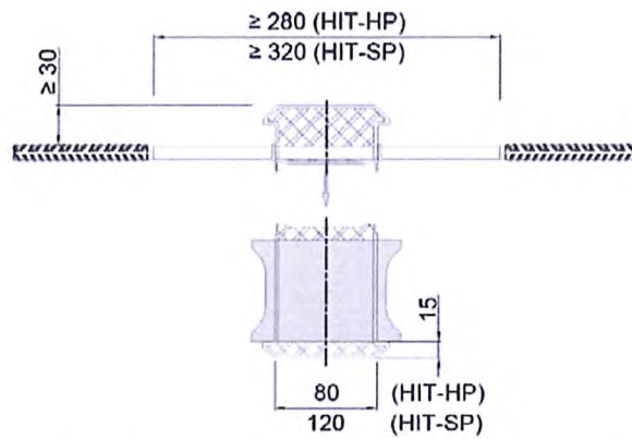
Figure 12: Halfen Insulated Connection HIT-HP/SP separated execution variation
