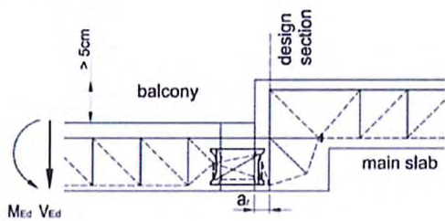
Figure 33: Strut-and-tie model HIT-HP/SP MVX-...-OD
