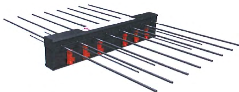
Figure 4: Halfen Insulated Connection HIT-HP/SP MVXL
