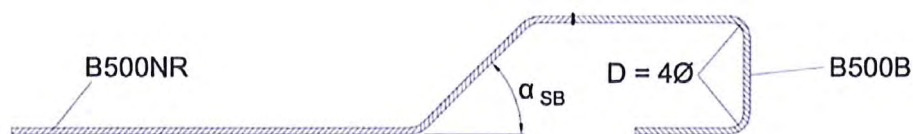
d) Execution with stainless reinforcing steel B500 NR, upper leg of shear bar carried out as loop made of B500B (embedment length of B500 NR of \geq 10 cm in the adjacent concrete)
