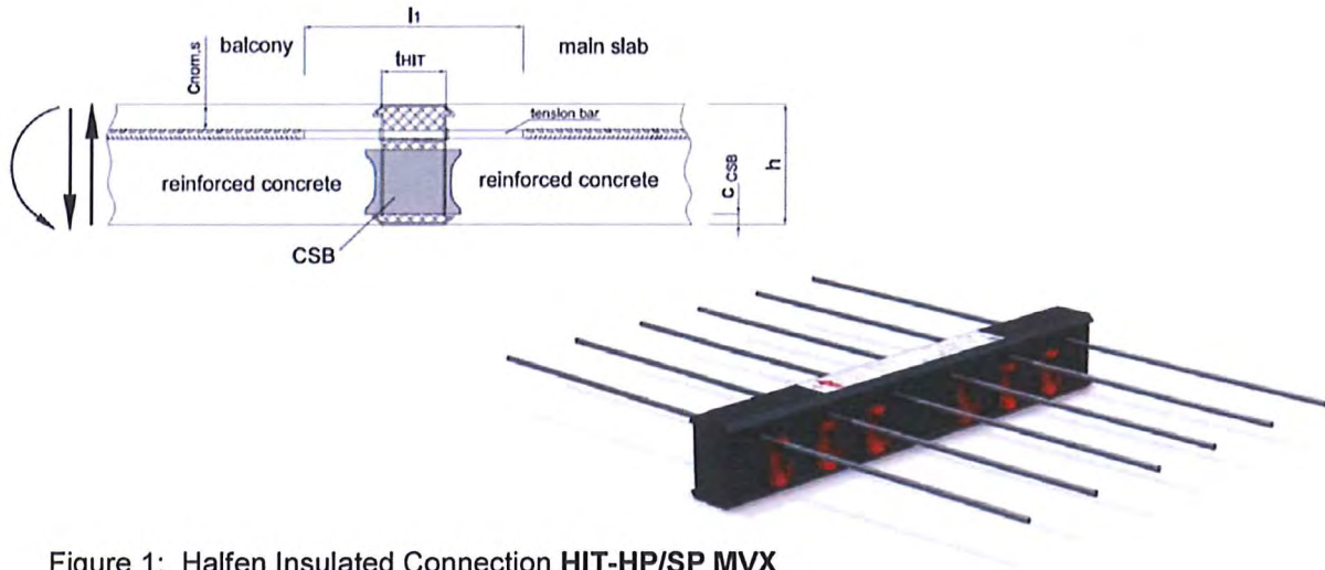
Figure 1: Halfen Insulated Connection HIT-HP/SP MVX
