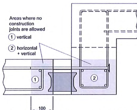
Figure 29: Reinforcement layout for Height offset HIT-HP/SP MVX_OD
