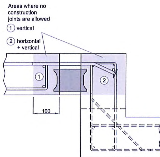
Figure 28: Reinforcement layout for height offset HIT-HP/SP MVX_OU
