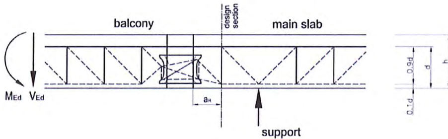
Figure 32: Strut-and-tie model and design section HIT-HP/SP MVX with compression shear bearing
